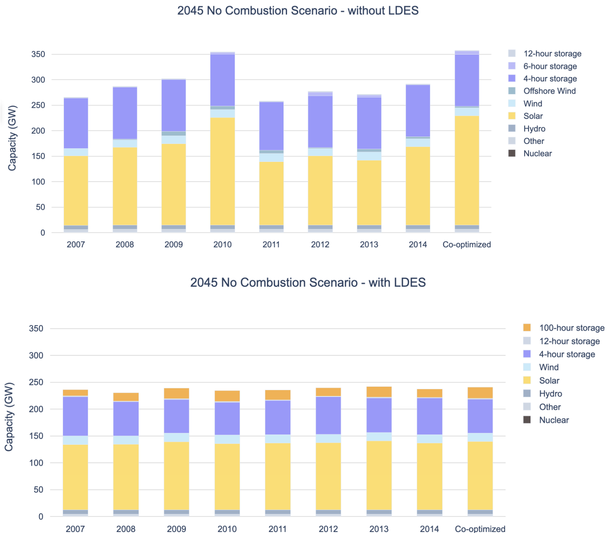
Figure 3. Variation in CAISO capacity expansion results across weather years
